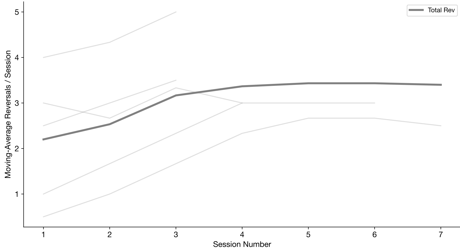
Moving-Average Total Reversals Over Time (n=5 subjects; sessions per subject=3–7; window=3)
